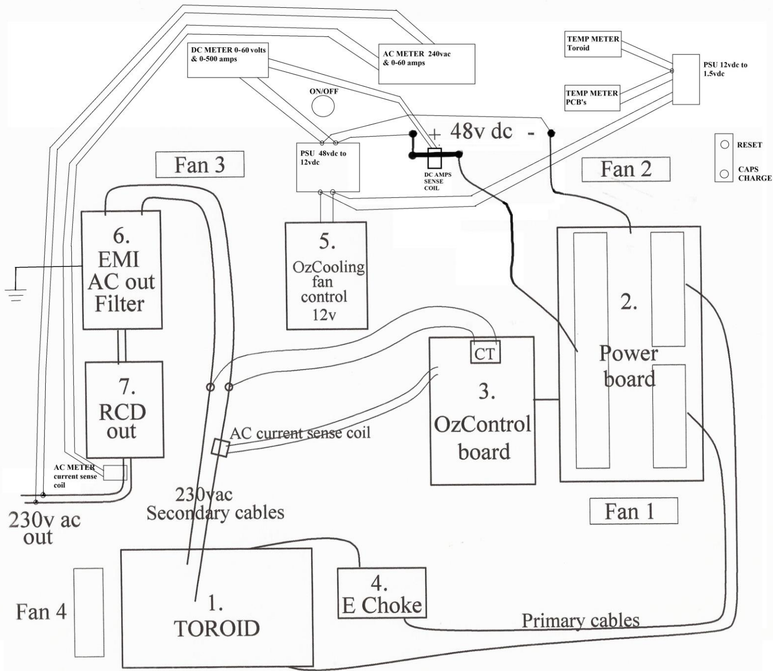
BLOCK DIAGRAM OZINVERTER ENCLOSURE
